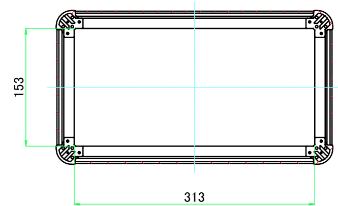
C-C (1:5)
